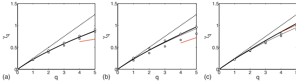
FIG. 5. (Color online) Same as Fig. 3 where this time the scaling exponents are plotted as function of q for \alpha=0.25\bar{h} so that \gamma_q=0.25q (dashed black line) [see Eq. (1)]. Also plotted \tilde{\gamma}_q [see Eq. (26)—thick solid black line] and \gamma'_q [see Eq. (35b)—thin solid black line]. A line in solid light gray (red) of slope equal to \alpha q/h_{\max} is plotted for large q [see also Eq. (32)].
