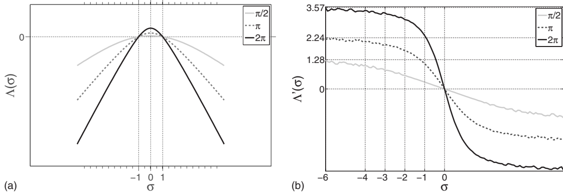
FIG. 1. (a) The function \Lambda(\sigma) corresponding to the alternating sine flow [Eq. (36)] for A = \pi/2, \pi, and 2\pi (where A = \pi U \tau, \tau = 1 and U varies). (b) The corresponding derivative of \Lambda(\sigma) .
